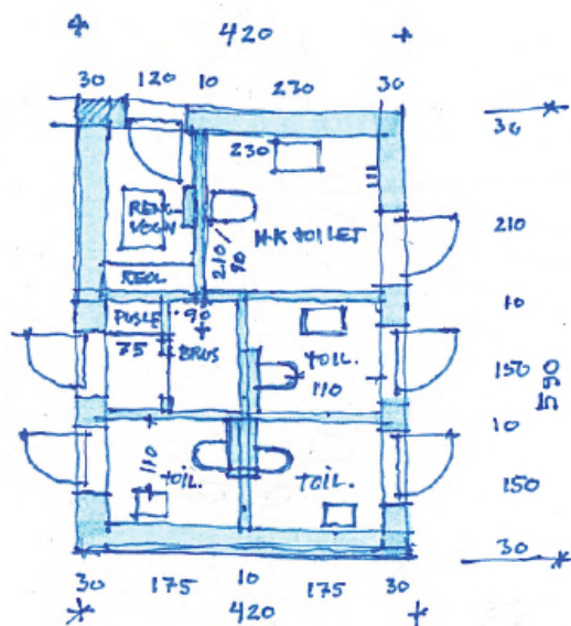
PLAN, TOILETBYGNING HVALPSUND 1:50
